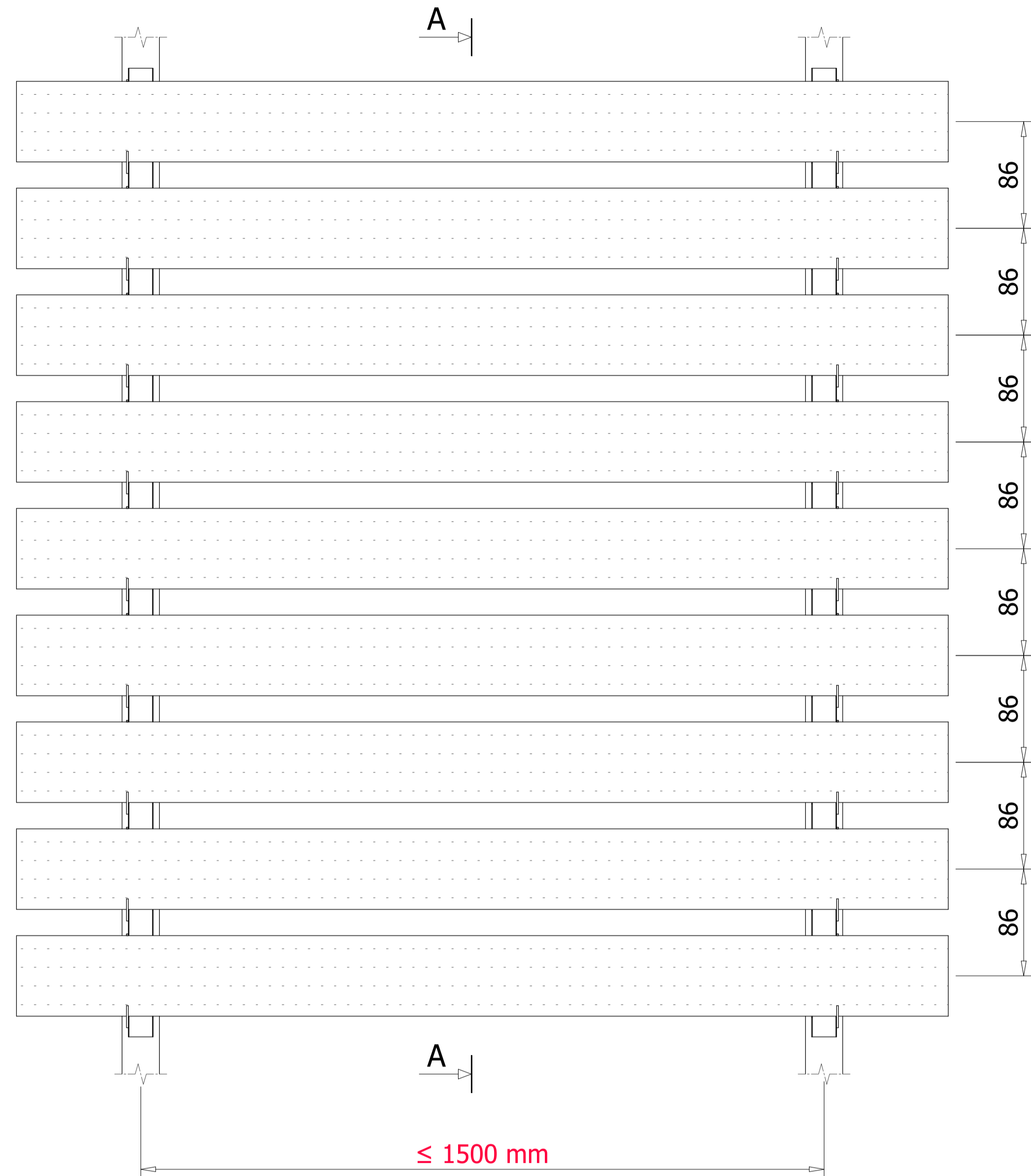
PANEL SECTION/ MẶT CẮT THANH LAM
